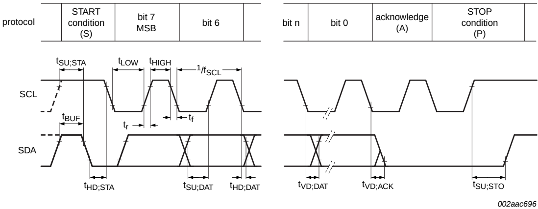
Fig 31. I 2 C-bus timing diagram
