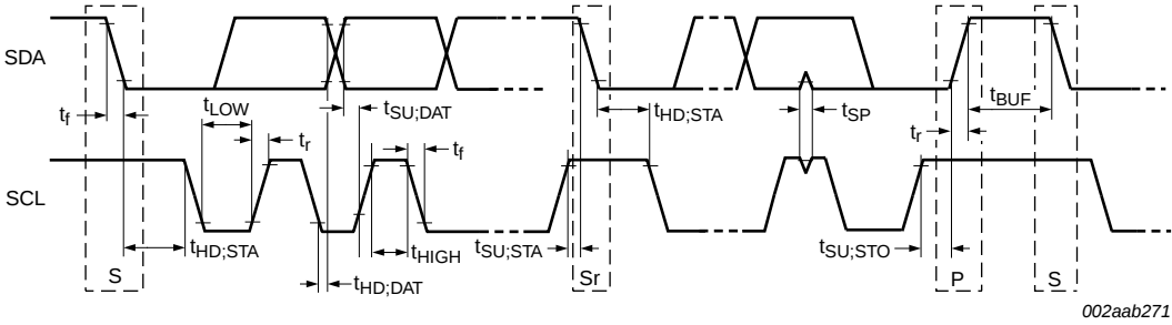
Fig 30. Definition of timing on the I 2 C-bus
