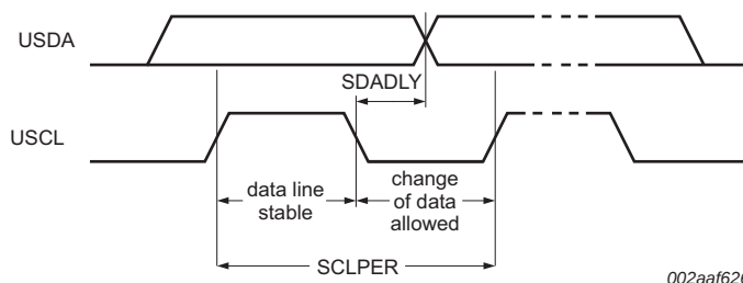
Fig 21. UFM I 2 C-bus bit transfer
