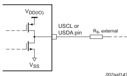
Fig 20. Simplified schematic of USCL, USDA outputs
