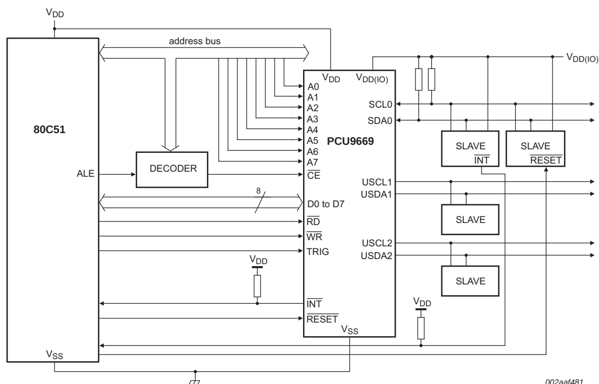
Fig 24. Application diagram using the 80C51
